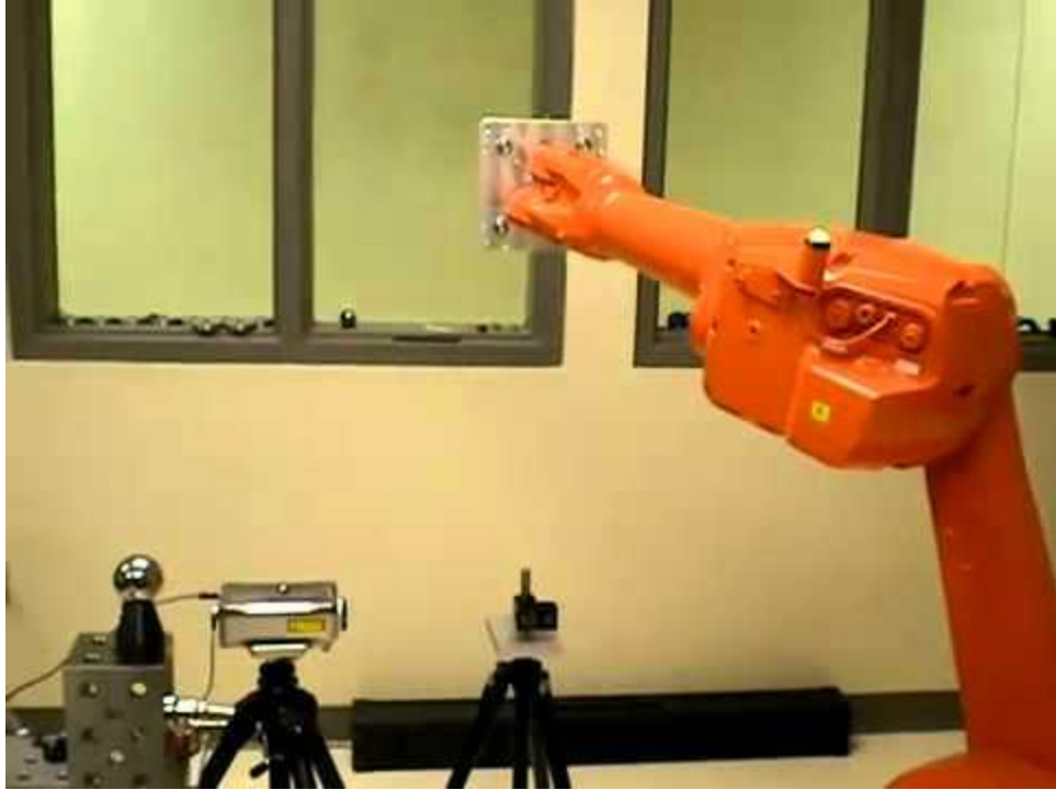
Laser Interferometer
